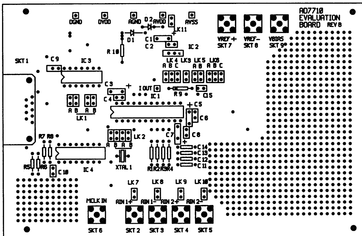
Figure 4. AD7710 Evaluation Board Silkscreen
